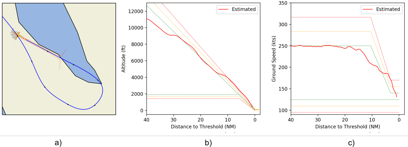
Figure 9. Illustration of the Asiana Airline Flight 214 crash. Figure a) represents the 2D trajectory, Figure b) illustrates the altitude profile, and Figure c) the ground speed profile. The plane is at 500ft ground level, its speed (c) and altitude (b) have returned to nominal values but its energy variation is atypical (with a coefficient of 0.97) and directs it towards an under-energy
