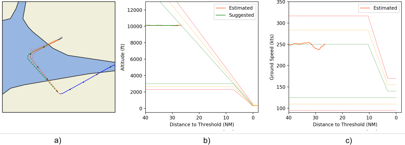
Figure 10. Illustration of the Pegasus Airline Flight 2193 crash. Figure a) represents the 2D trajectory, Figure b) illustrates the altitude profile, and Figure c) the ground speed profile. The plane turns in base leg (a). Its ground speed increases (c) and it passes over the glide path (b). The tool suggests to slightly lengthen the track (in green).
