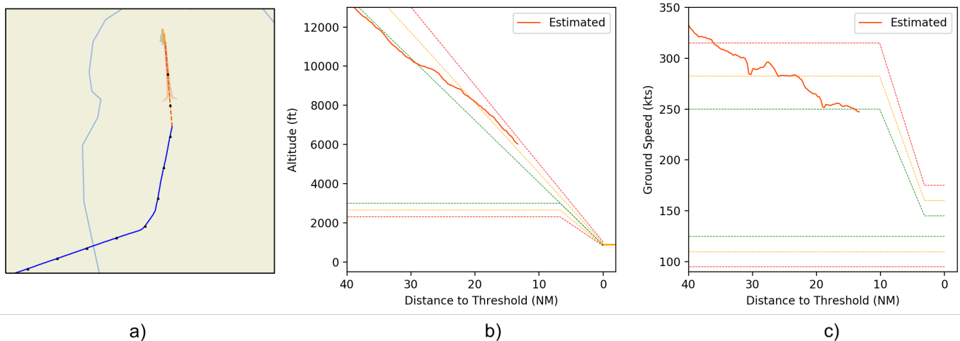
Figure 15. Illustration of the Hermes Airline Flight 7817 crash. Figure a) represents the 2D trajectory, Figure b) illustrates the altitude profile, and Figure c) the ground speed profile. The aircraft intercepts the runway extended centerline. The deviation of 10^\circ right, shortened the track a), the plane is now above the glide path b). The aircraft's ground speed is around 250kts (c). The tool indicates an atypical situation due to an excess of potential energy.
