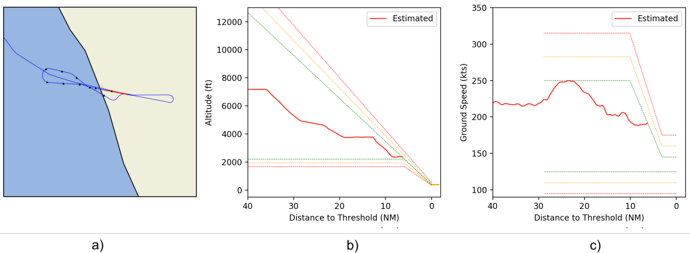
Figure 19. Air India Express Flight 1344 lateral, altitude and speed profiles. The altitude profile is nominal however, its ground speed is around 200kts with no sign of reduction. The atypical coefficient has increased up to 0.97 underlying an atypical variation leading the aircraft to high energy.
