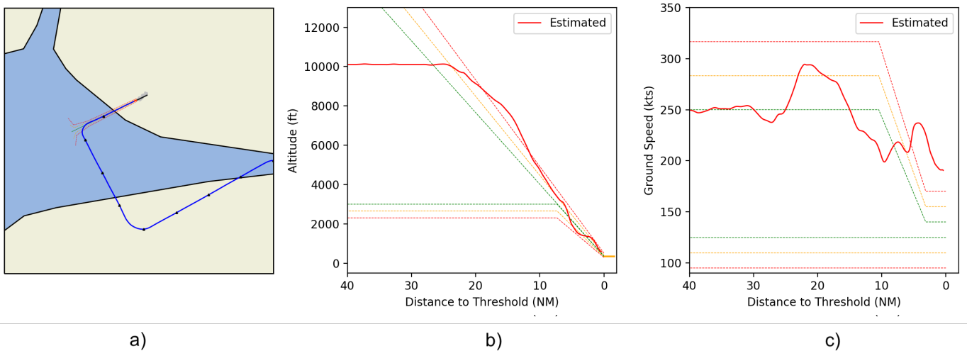
Figure 13. Illustration of the Pegasus Airline Flight 2193 crash. Figure a) represents the 2D trajectory, Figure b) illustrates the altitude profile, and Figure c) the ground speed profile. The aircraft is 1NM from the runway threshold. The glide path management presents large variations, its ground speed is 190kts the atypicality did not decrease throughout the final.
