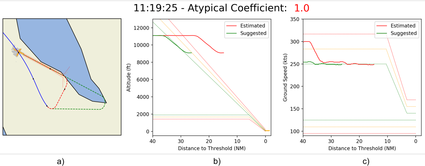
Figure 6. Illustration of the Asiana Airline Flight 214. Figure a) represents the 2D trajectory, Figure b) illustrates the altitude profile, and Figure c) the ground speed profile. The plane is here in downwind leg (a). The tool indicates that a direct to the interception chevrons is critical (in red) and would cause the plane to be in over-energy due to high potential energy figure (a). The tool suggests a trajectory extending the tailwind leg (in green).
