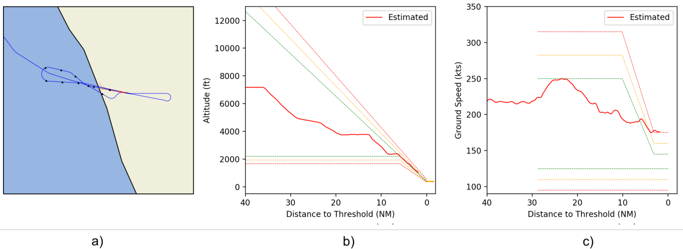
Figure 21. Air India Express Flight 1344 lateral, altitude and speed profiles. The ADS-B data stopped at 1.6NM to the runway threshold. The aircraft is still on the glide path. However, the ground speed is not reducing anymore and stagnates at 175kts. The atypical coefficient increased up to 0.96 again underlying a high kinetic energy
