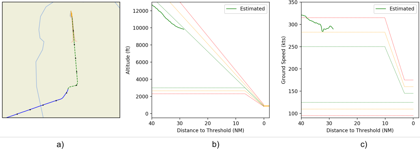
Figure 14. Illustration of the Hermes Airline Flight 7817 crash. Figure a) represents the 2D trajectory, Figure b) illustrates the altitude profile, and Figure c) the ground speed profile. The crew follows the localizer interception heading given by the Air Traffic Controller and requests permission to deviate its trajectory by 10^\circ left to avoid a cloud a). The aircraft's ground speed is slightly high (c) and it is still under the glide path (b). The tool indicates that the aircraft is in a typical situation.
