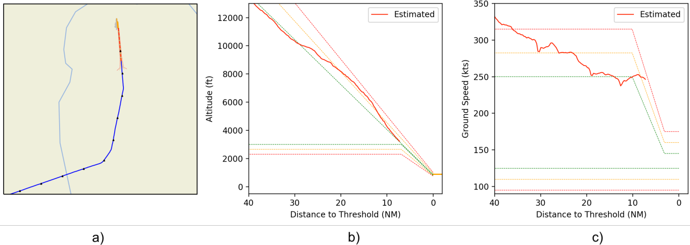
Figure 16. Illustration of the Hermes Airline Flight 7817 crash. Figure a) represents the 2D trajectory, Figure b) illustrates the altitude profile, and Figure c) the ground speed profile. The plane has just recovered the glide path a). However, the potential energy b) has been transformed into kinetic energy and there is a slight increase of the ground speed towards 260kts c). The atypicality increases around 0.88 due to an excess of kinetic energy.
