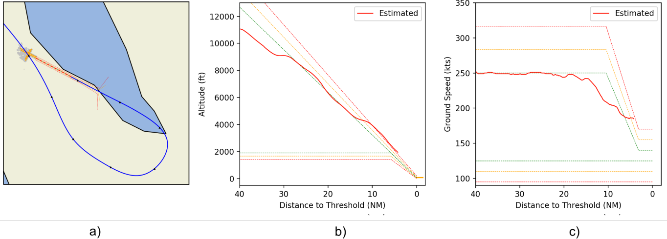
Figure 8. Illustration of the Asiana Airline Flight 214 crash. Figure a) represents the 2D trajectory, Figure b) illustrates the altitude profile, and Figure c) the ground speed profile. The aircraft is 5NM from the runway threshold (a), above the glide path (b) with a ground speed of 180kts due to air traffic constraints (c). The plane is in over-energy due to both high potential and kinetic energy.
