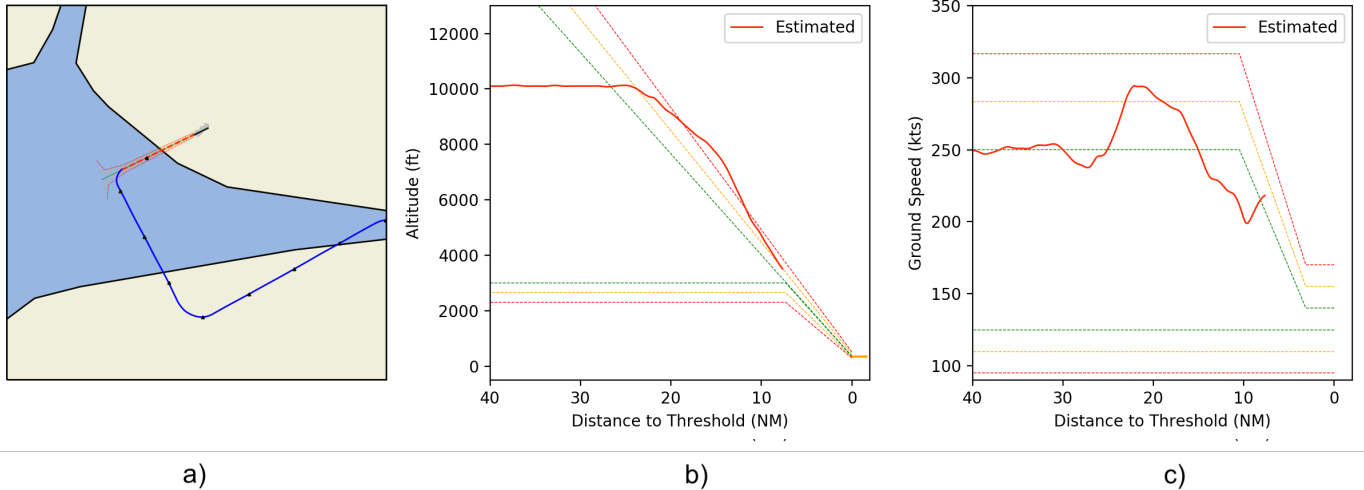
Figure 12. Illustration of the Pegasus Airline Flight 2193 crash. Figure a) represents the 2D trajectory, Figure b) illustrates the altitude profile, and Figure c) the ground speed profile. The plane is on final approach (a), it is high on the glide path (b). Its ground speed is increasing (c) and its atypical score is 0.87.
