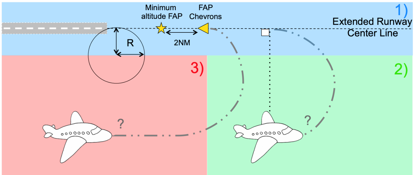
Figure 4. Illustration of the different cases of the methodology. different situation. Case 1) in blue, corresponds to the portions of the trajectory where the aircraft is on the localizer (distance to the localizer less than one turning radius). Case 2) in green, corresponds to the portions of trajectory where the aircraft is at on base or downwind leg but beyond the perpendicular to the chevrons. Case 3) in red, corresponds to the portions of trajectories where the aircraft is in downwind leg, before the perpendicular to the chevrons.
