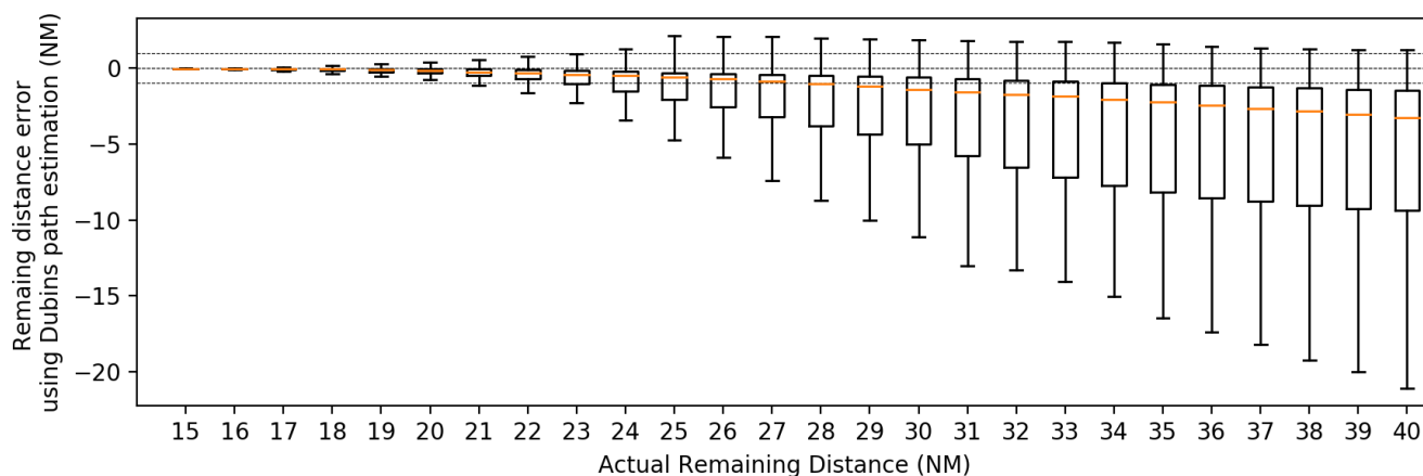
Figure 5. Box plot of the difference between estimated and real remaining distance between 15NM and 40NM (computed every 1NM over 1600 radar trajectories)
