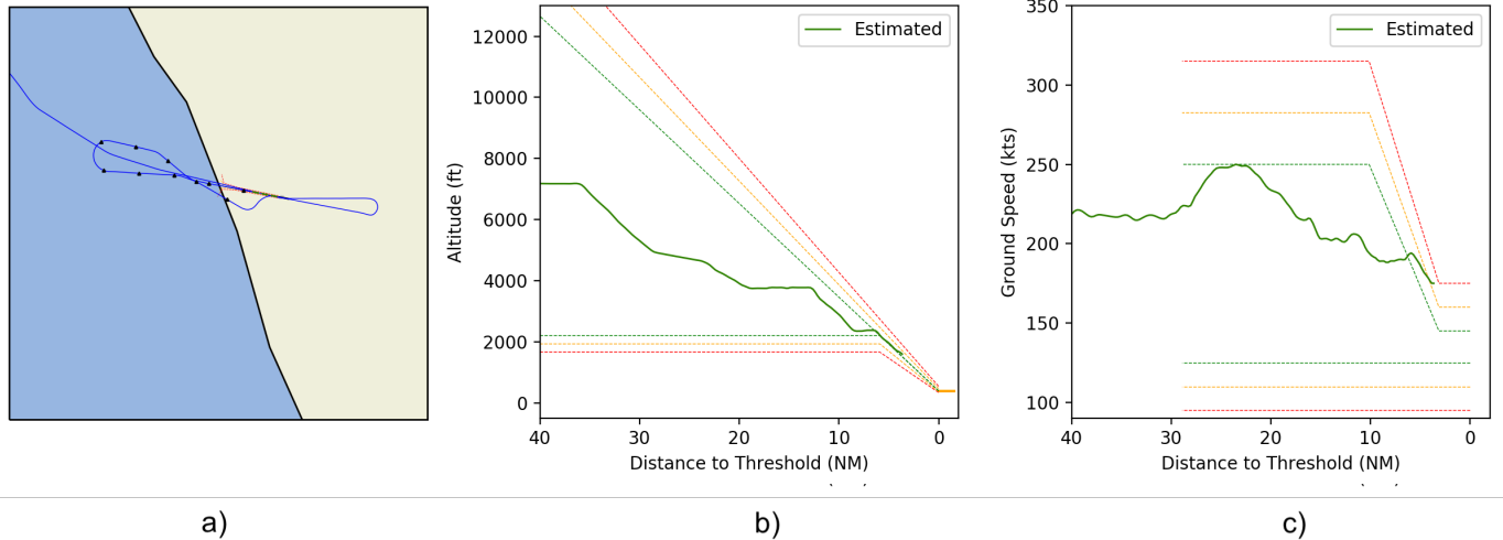
Figure 20. Air India Express Flight 1344 lateral, altitude and speed profiles. The aircraft descends on the glide path, the ground speed has started to reduce down to 175kts. The atypical coefficient is back to green areas(0.09). The reduction of the energy returns the aircraft to a less atypical state
