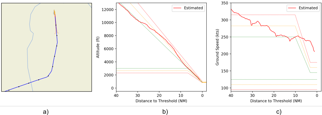
Figure 17. Illustration of the Hermes Airline Flight 7817 crash. Figure a) represents the 2D trajectory, Figure b) illustrates the altitude profile, and Figure c) the ground speed profile. The aircraft is about 3NM from the runway threshold a). Its atypicality peaks at 1.0 because of a very high ground speed of 210 kts c), although decreasing. The aircraft is not stabilized with a very high speed and nevertheless continues its approach.
