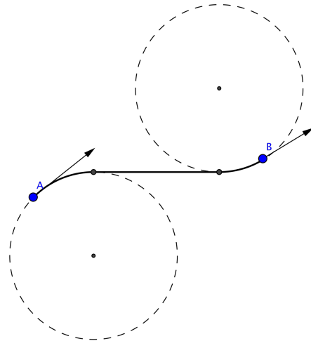
Figure 3. Illustration of a Dubins path between two points A and B. The solution here is RSL: a right turn, then a straight line, and finally a left turn.
