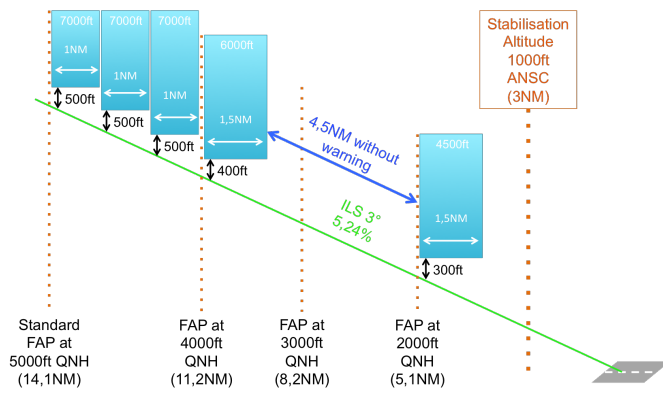
Figure 1. Illustration of the Glide Interception From Above detection implemented at Charles de Gaulle airport. 3D volumes have been set up to detect when an aircraft is too high on the glide path. A recovery plan is proposed. If it is still too high on the glide path further downstream, the air traffic controllers suggest a go-around.
