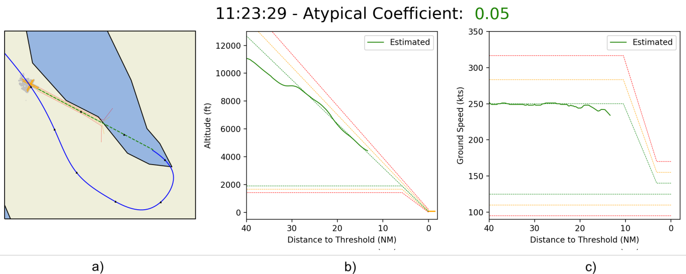
Figure 7. Illustration of the Asiana Airline Flight 214 crash. Figure a) represents the 2D trajectory, Figure b) illustrates the altitude profile, and Figure c) the ground speed profile. The plane has just intercepted the runway centerline (a) and is in good condition, it is on the glide path (b) and presents a nominal speed (c).
