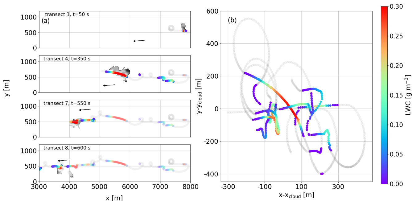
Figure 14. (a) Trajectories of exploration by following cloud N2 for four different transects. The colors represent the measured LWC, and the gray surface corresponds to the cross section of reference cloud N2 for the different times. The shading colors correspond to the past transects. The black arrow represents the direction of the advective wind. (b) Measured LWC in cloud frame during the exploration. The colored lines correspond to the values of measured LWC exceeding 10^{-2} \text{ g m}^{-3} , and the gray lines correspond to the measured LWC below this threshold.
