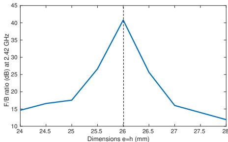
Fig. 2: Variation of the dimensions d = f vs. F/B ratio at 2.42 GHz.
