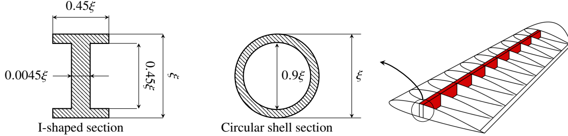
Fig. 7 Wing Spar Cross Sections
