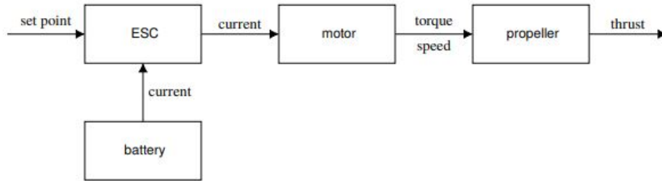
Fig. 2 Multirotor Propulsion Group [11]
