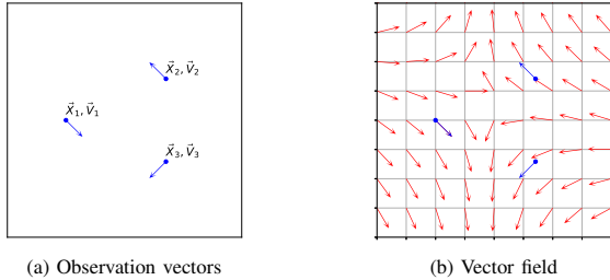
Figure 2. Measurement or observation vectors and vector fields derived by the linear dynamical model
