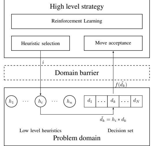
Figure 6. Adaptive metaheuristic framework with three major components: (i) low-level heuristics, (ii) heuristic selection, (iii) reinforcement learning and (iv) move acceptance and (iv)
