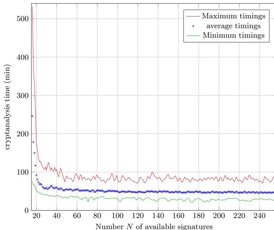
Fig. 6: Execution timings (min) for breaking PARA-2 as a function of the number N of signatures available to the adversary. Timings were averaged over a hundred executions.
