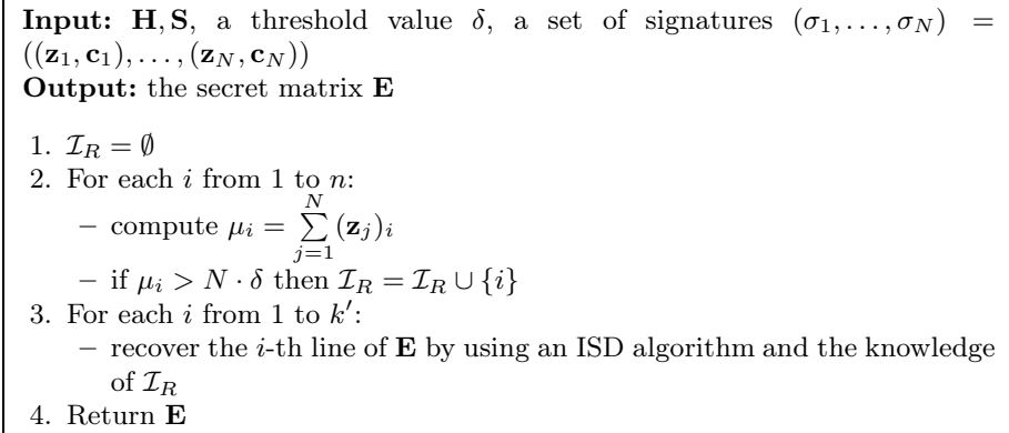
Fig. 4: Private key recovery of the SHMWW scheme
