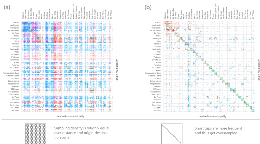
Figure 8. Zone-level OD matrix of XDR (a) and survey (b) flows for the night valley period. Sparser measures and an over representation of intramunicipal flows can be appreciated in the survey.
