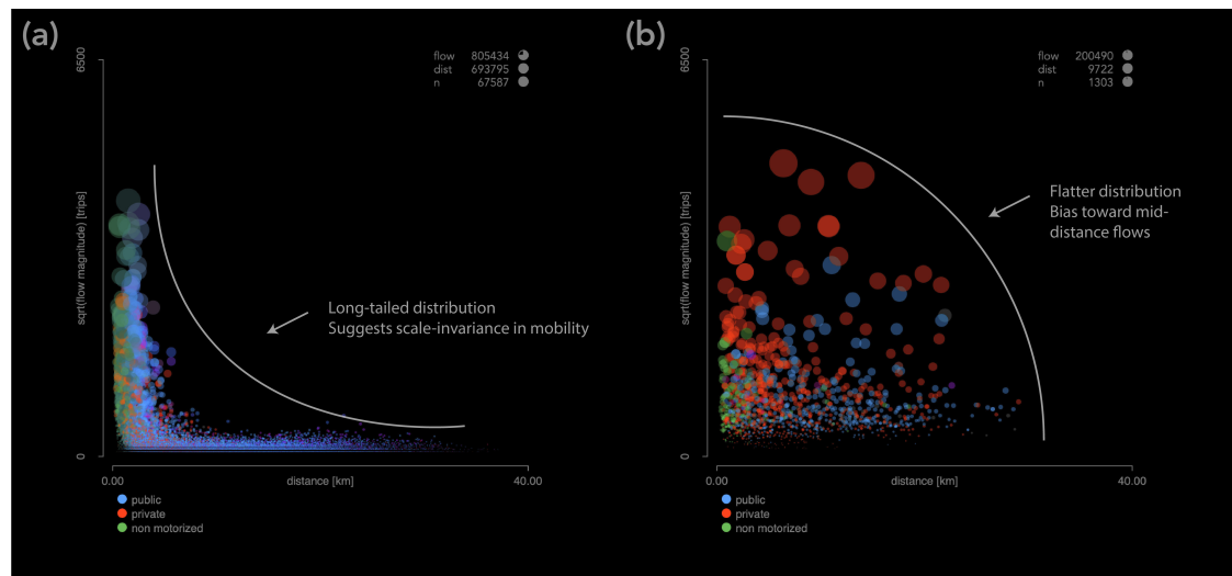
Figure 5. Pervasive (a) and survey (b) flows at night time. Each circle is an origin-destination pair, its area the flow magnitude, with color coded mode split. Highlighted are the different overall shapes present in their distribution.
