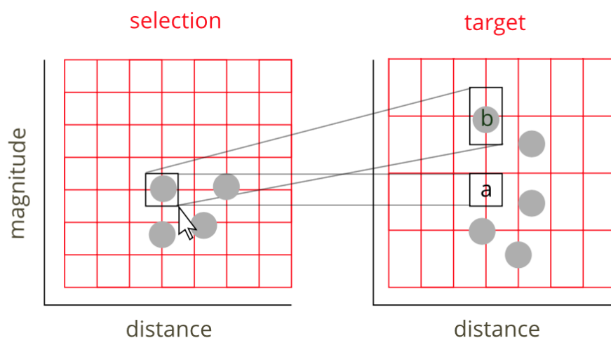
Figure 3. Selection over different datasets in the scatterplot is facilitated by our distribution-aware selection tool. A range selected in one scatterplot is not merely transposed to a , which would probably end in an empty selection, but linearly transformed into b , according to the grid automatically defined based on the distribution of each dataset.
