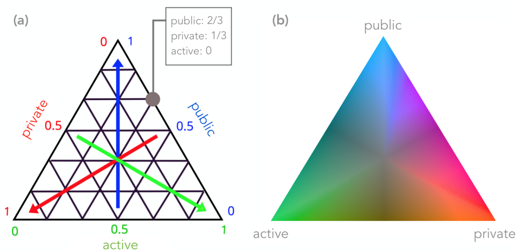
Figure 2. Ternary color scale construction schema (a) and resulting colormap (b) used to encode mode split across views.
