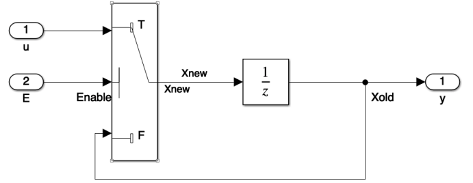
Figure 6: Simulink model for requirement [AP-003c-v4]
