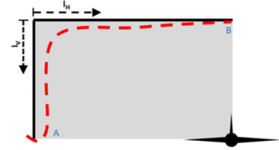
Figure 5: Side view of an intrusion. The red dashed line shows the intrusion path of an aircraft through the protected zone of another.
