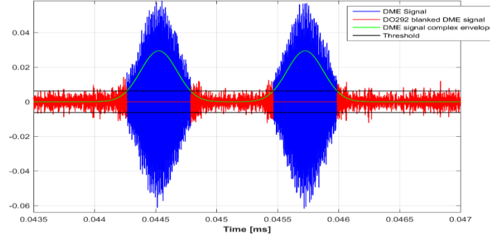
Figure 5: Example of the behavior of the DO-292 instantaneous blanker over the signal complex envelope
