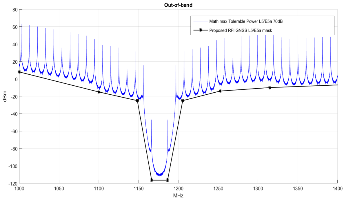
Figure 10: L5/E5a GNSS out-of-band RFI mask
