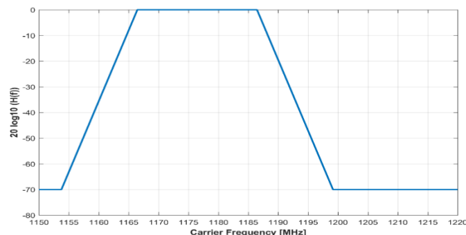
Figure 4: RFFE plus antenna equivalent transfer function defined in DO292 customized for a BW=20MHz
