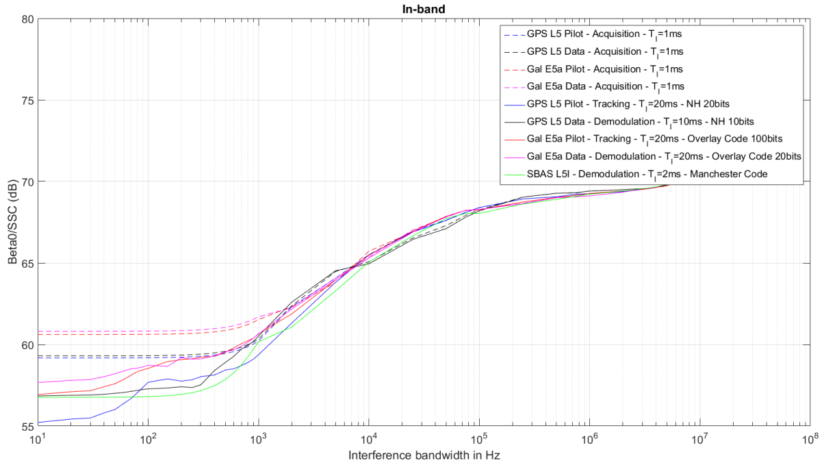
Figure 8: Local replica PSD filtered by the integrate and dump filter
