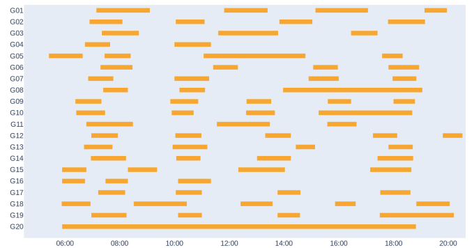
Figure 2. Gantt diagram of an optimal solution to an instance with 20 gates and 78 aircraft at terminal J of Paris-CDG airport.
