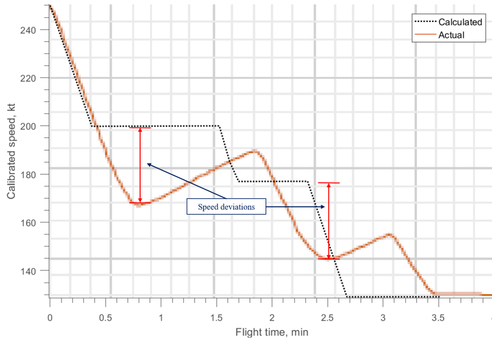
Fig. 10 Test 1: Comparison between the speed profile calculated and the actual one flown in flight simulator.
