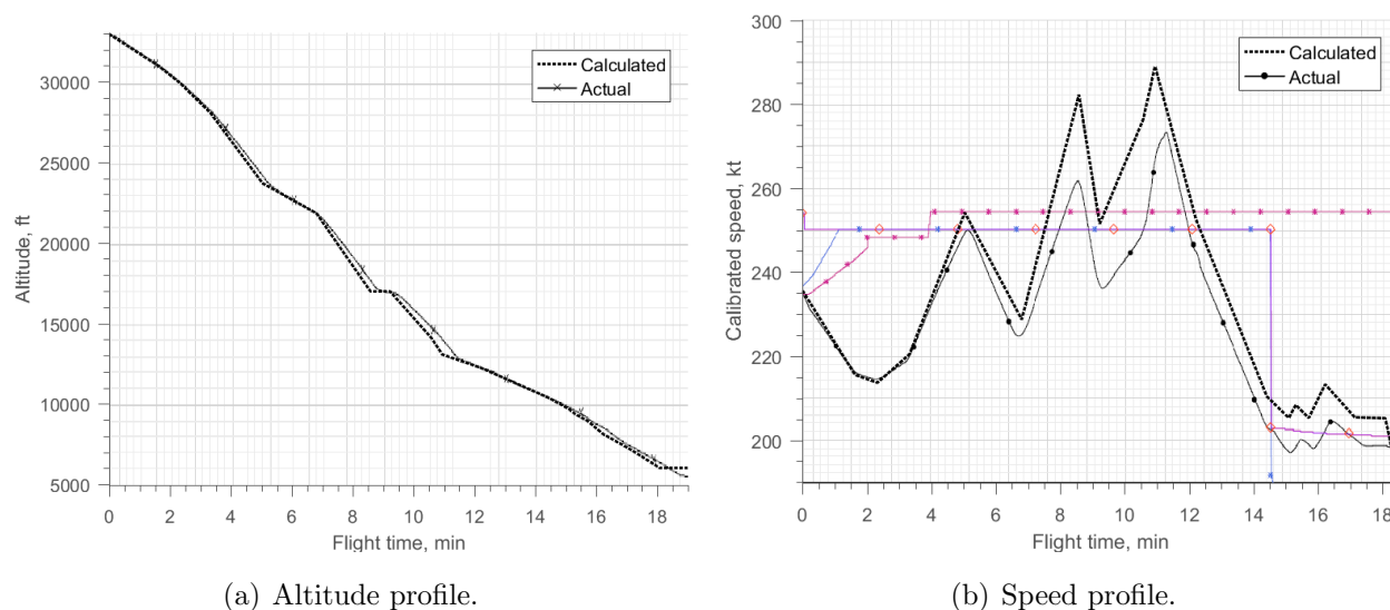
Figure 6. Trajectory comparison between A* calculation and simulator flight.
