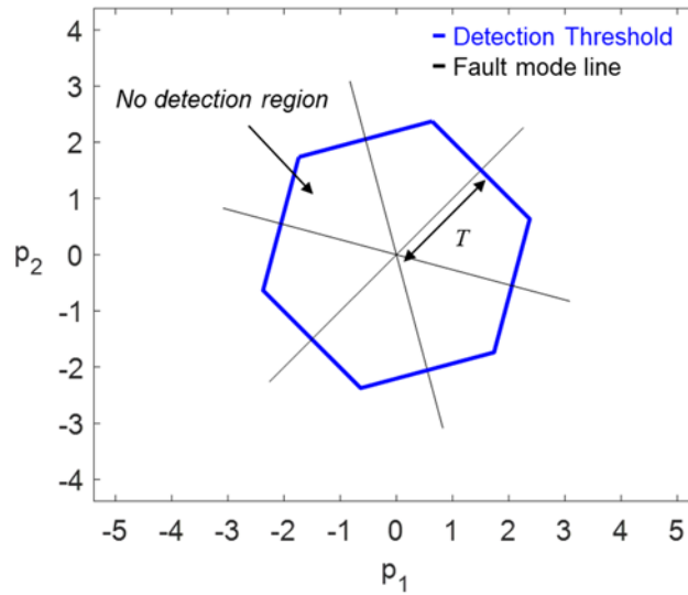
Fig. 1 Fault detection boundaries for the solution separations in the parity space
