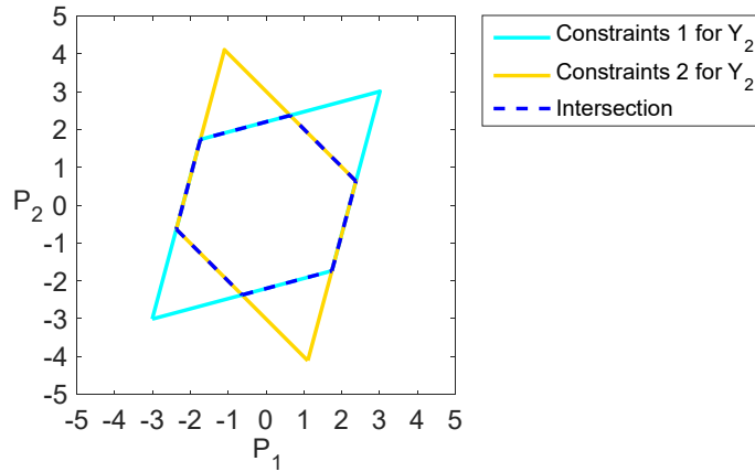
Fig. 2 Detection boundaries (yellow and light blue parallelograms) defined by two constraints on the new random variable ( y_2 ) after the transformation in the parity space. A single constraint on y_2 , the intersection of two regions, is the same as the detection bounds based on the parity vector (dotted blue hexagon)
