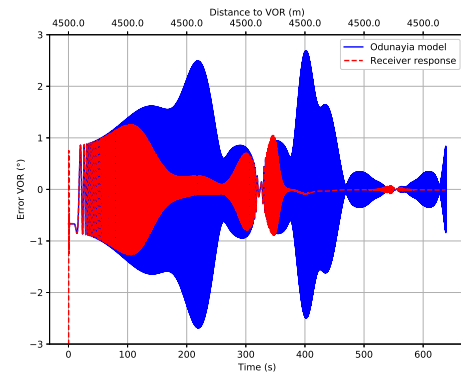
Fig. 5. Receiver response.
