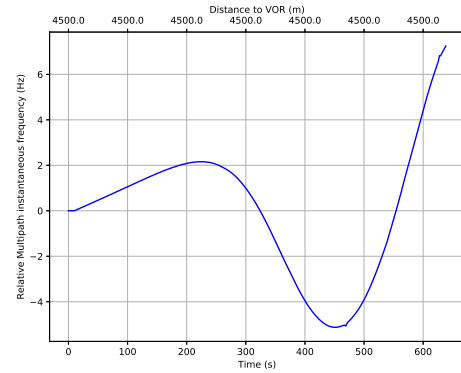
Fig. 4. Relative multipath instantaneous frequency.
