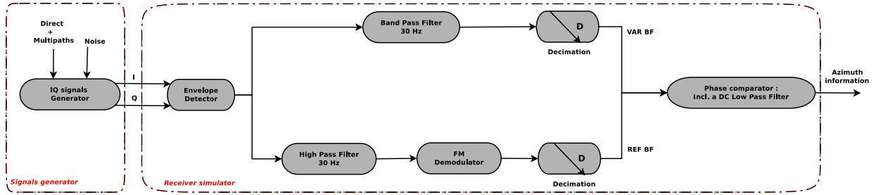
Fig. 2. Block diagram of the VOR receiver.
