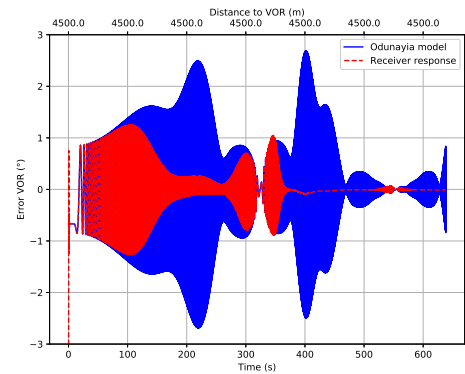
Fig. 5. Receiver response.
