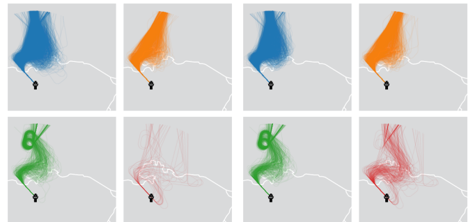
Figure 13. Clusters identified by DCEC for one flow with \lambda = 0 (left) and \lambda = 0.5 (right); to be related with the second line of the grid in Figure 11
