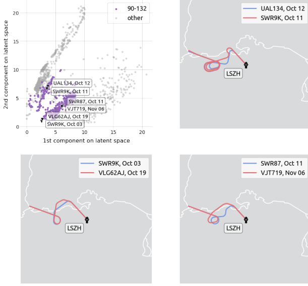
Figure 3. The scatter plot displays the latent space on trajectories containing one or several loops. Sample that are close to each other reveal similar patterns on the map. In particular, trajectories stacking holding patterns are plotted on the top right in purple and the subset of trajectories corresponding to strictly more than one holding pattern are located in the top left purple cluster.
