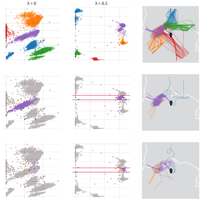
Figure 9. Comparison of latent spaces for artefact with \lambda = 0 , \lambda = 0.5 , and corresponding samples on the right. Colours are consistent with initial flows in the beginning of the paper.
