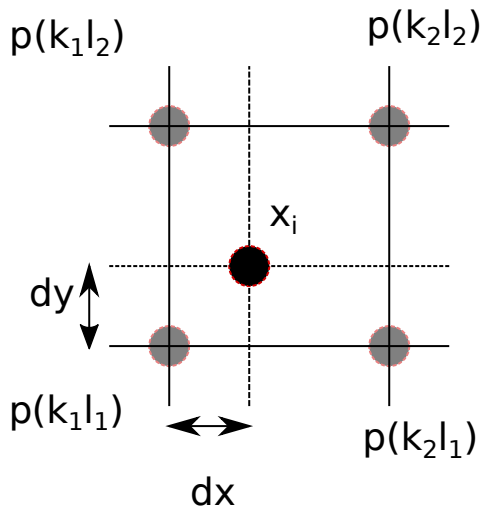
Fig. 1. Bilinear interpolation
