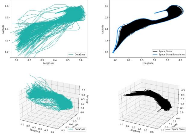
Figure 2. State Space
