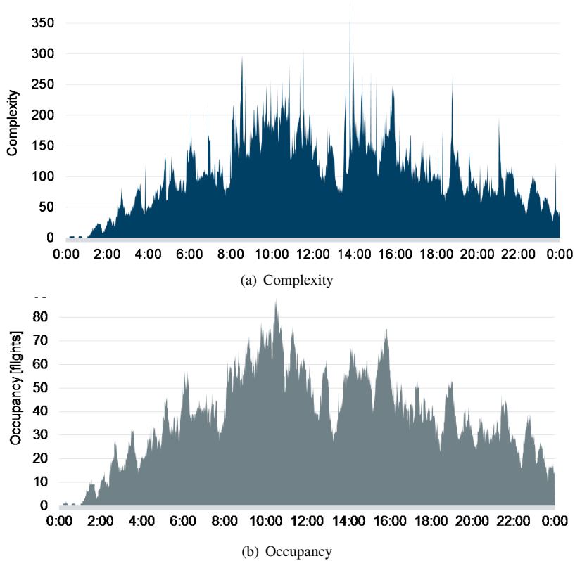
Fig. 3: Demand of the ACC LHCCCTA
