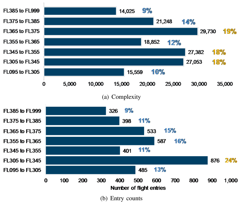
Fig. 4: Demand per vertical layers
