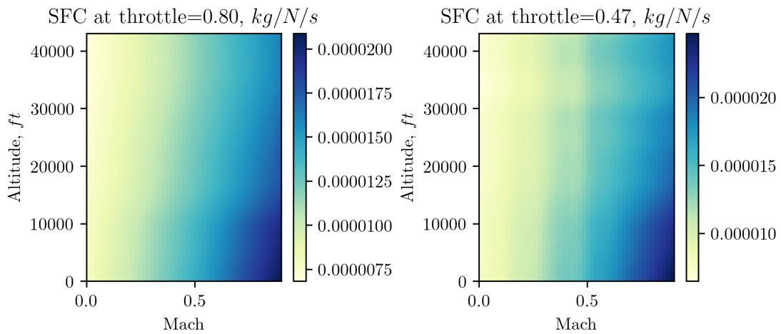
Fig. 8 Specific fuel consumption with respect to Mach number and altitude by RMTC
