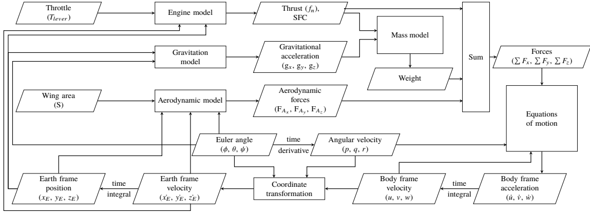
Fig. 4 Data flow and computational procedure of mission analysis
