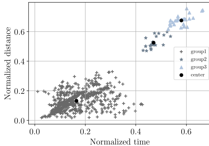
Fig. 5 Clustering results from the DBSCAN algorithm, \epsilon = 0.06 and the number of minimum samples = 14.
