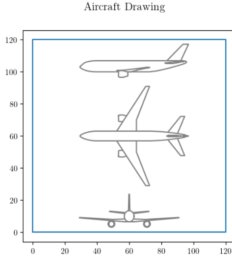
Fig. 10 The drawing results from MARILib.
