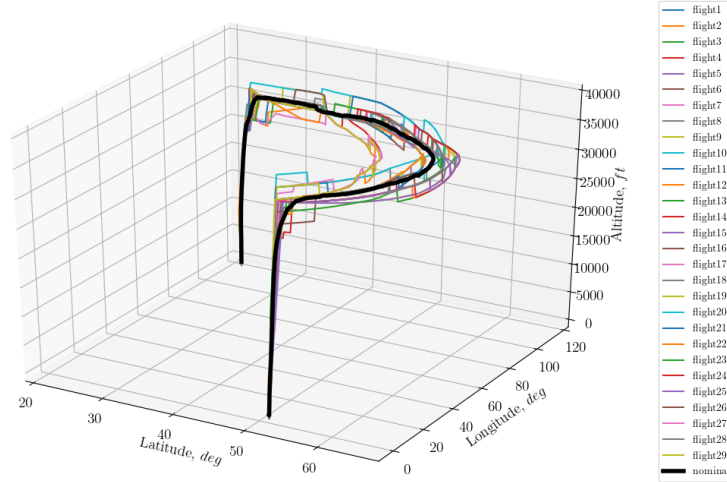
Fig. 6 Reference route for TLARs and flight scenario
