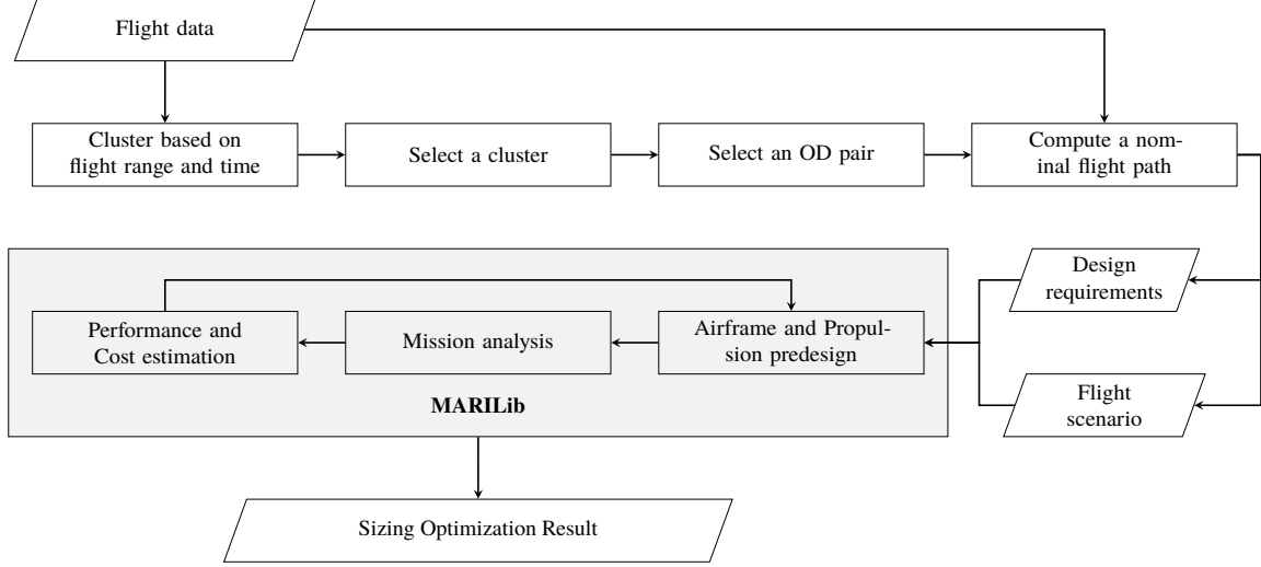
Fig. 1 Flow chart of proposed research
