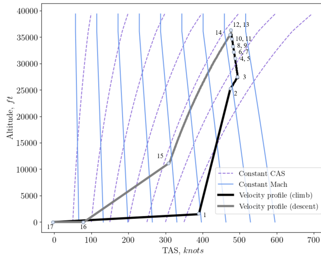
Fig. 7 Velocity profile for the mission analysis
