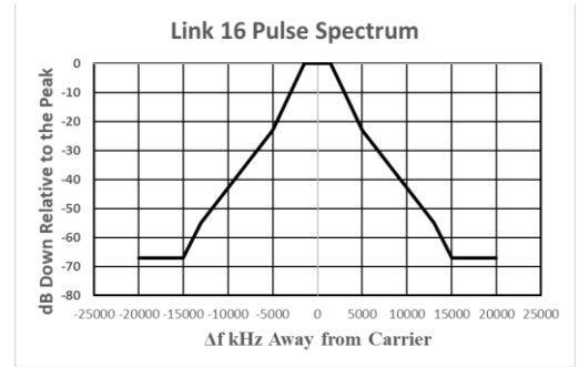
Fig. 11. JTIDS/MIDS Pulse Spectrum Model [1]
