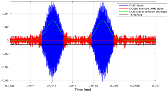
Fig. 3. Example of the behavior of the DO-292 instantaneous blinder over the signal complex envelope
