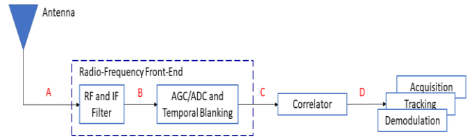
Fig. 1. Generic civil aviation GNSS receiver block scheme
