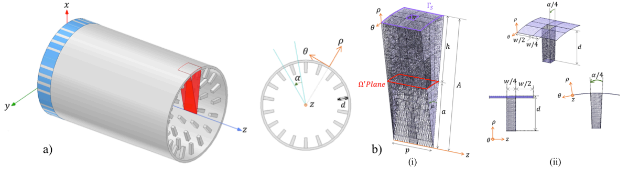
Figure 9. a) Waveguide with the peak-structure metamaterial. The 3-D blue dashed section is used in HFSS, and the 3-D red part is used in the MET b) represented with the mesh. The dimensions are (i) A = 30 mm, a = 15 mm, h = 15 mm, p = 10 mm; (ii) for the \Gamma_S part (the PEC boundary) of the 3-D unit cell with d = 8 mm, \alpha = 20^\circ , and w = 8 mm.
