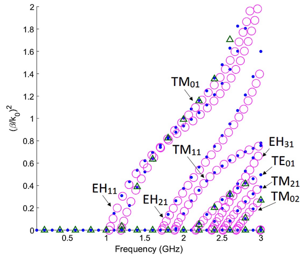
Figure 6. Dispersion diagrams of the cylindrical waveguide with the corrugation presented in Fig. 5a) obtained with the MET + 3-D FEM code (dots), the MET + 2-D FEM code [31] (triangles) and HFSS (circles).
