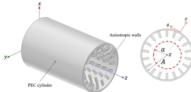
Figure 1. Cylindrical waveguide with anisotropic walls.
