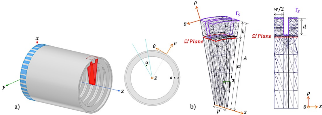
Figure 5. a) Corrugated waveguide. The 3-D blue dashed section is used in HFSS, and the 3-D red part is used in the MET b) represented with the mesh. The dimensions are A = 100 mm, a = 80 mm, h = 20 mm, p = 26.225 mm, w = 20.98 mm, d = 18.2 mm and \alpha = 20^\circ .
