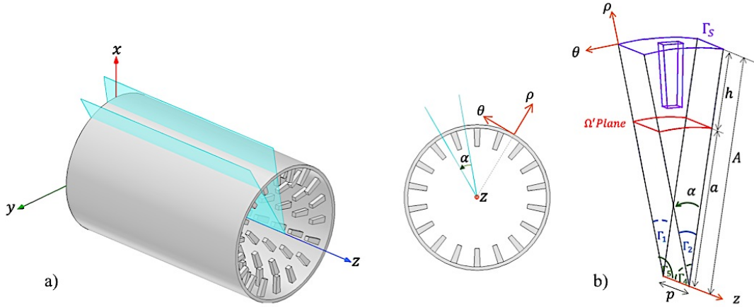
Figure 3. a) 3-D metamaterial waveguide and b) the 3-D unit cell.
