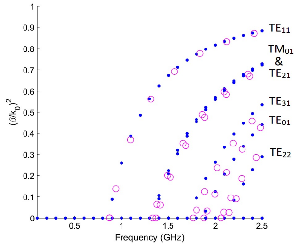
Figure 8. Dispersion diagrams of the cylindrical waveguide with the corrugation presented in Fig. 7a) obtained with MET (dots) and HFSS (circles).
