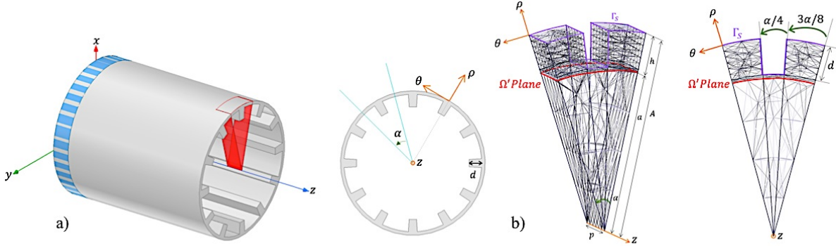
Figure 7. a) Corrugated waveguide along the z-axis. The 3-D blue dashed section is used in HFSS, and the 3-D red part is used in the MET b) represented with the mesh. The dimensions are A = 100 mm, a = 80 mm, h = 20 mm, p = 26.225 mm, d = 18.2 mm and \alpha = 30^\circ .
