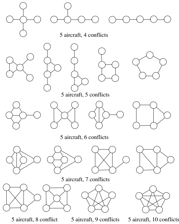
Fig. 3 Different structures for 5 aircraft clusters. Each vertex represents an aircraft, each edge is a conflict between two aircraft.
