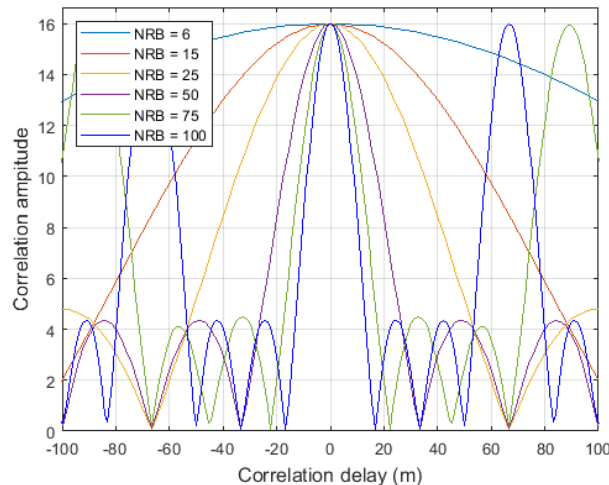
Figure 8. PCFICH autocorrelation amplitude as a function of the correlation delay for a different number of resource blocks. Notation: NRB, total number of downlink resource blocks
