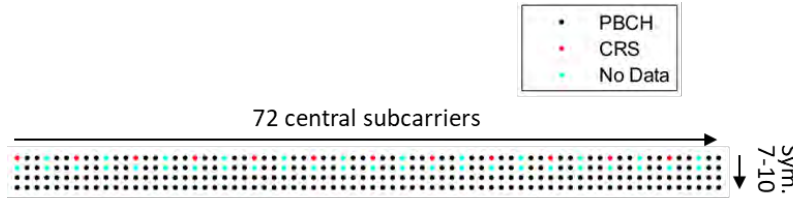
Figure 4. An example of data symbols allocated within the central 72 resource elements of the system bandwidth to antenna port number zero with two antenna ports configuration
