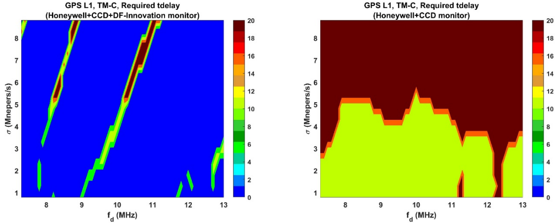
Fig. 14-Required tdelay for the PMD compliance for the TMC under GPS L1 fault mode (left: with DF-Innovation monitor, right: without proposed monitor)
