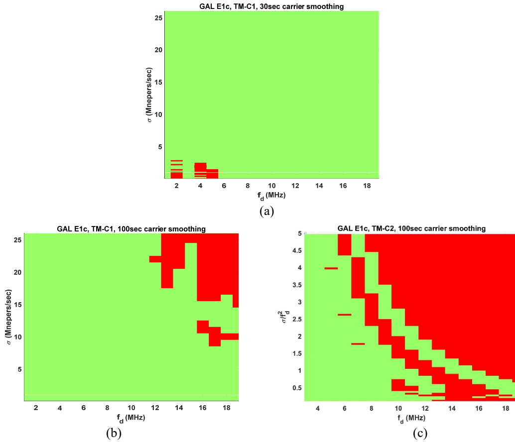
Fig. 12-Noncompliant region in the threat space for Galileo E1c: (a) TMC1, 30-second time constant, (b) TMC1, 100-second time constant and (c) TMC2, 100-second time constant
