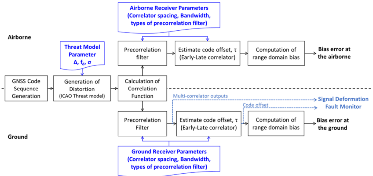
Fig. 8-Diagram of the fault generation process
