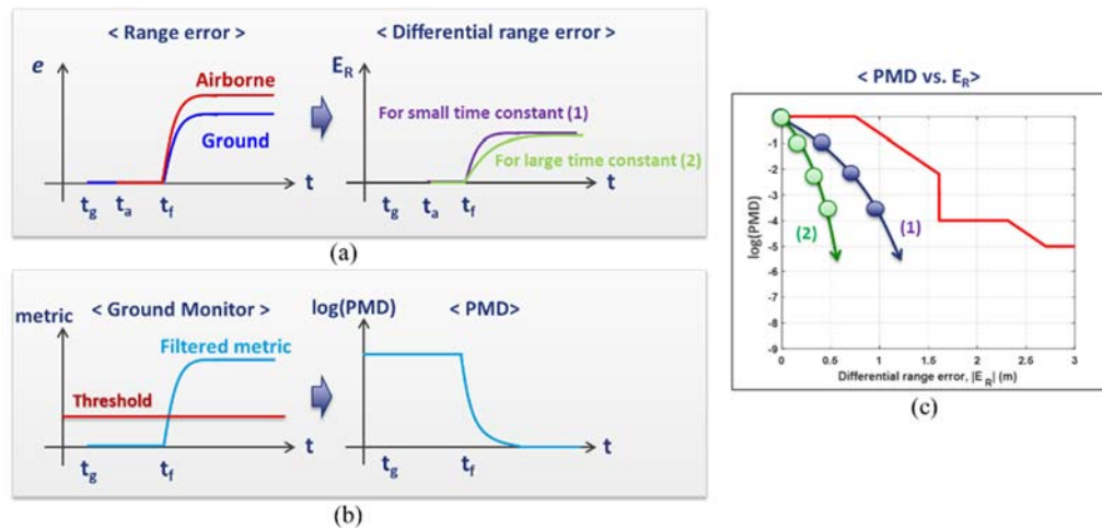
Fig. 9-Description of post-convergence case and the effect of time constant of carrier smoothing for the PMD compliance: (a) Range errors at ground and airborne and associated differential range error, (b) Ground monitor and corresponding PMD and (c) The PMD compliance curve for small and large time constants of the smoothing filter (red line: the PMD requirement)
