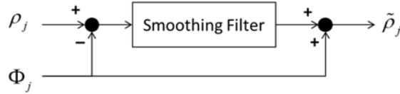
Fig. 1-Carrier smoothing in dual-frequency modes for the DF-Innovation Monitor
