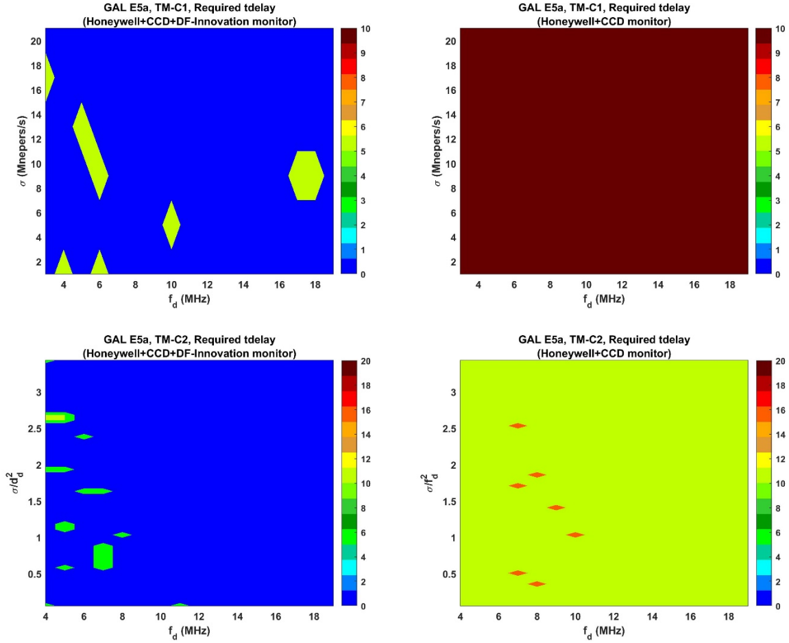
Fig. 16-Required t_{delay} for the PMD compliance for the TMC1 under Galileo E5a fault mode in the upper panel and TMC2 in the lower panel (left column: with the DF-Innovation monitor, right column: without the proposed monitor)
