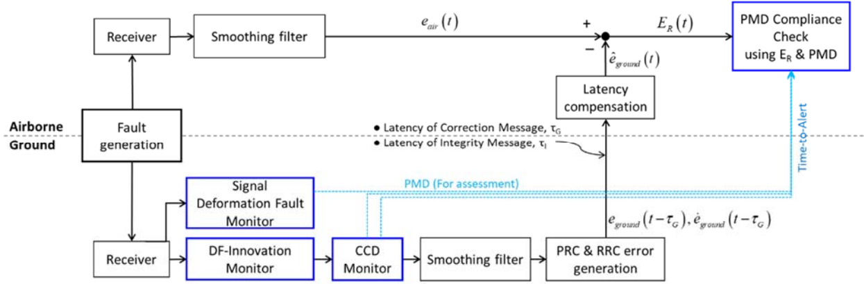
Fig. 7-Overall process of the PMD assessment
