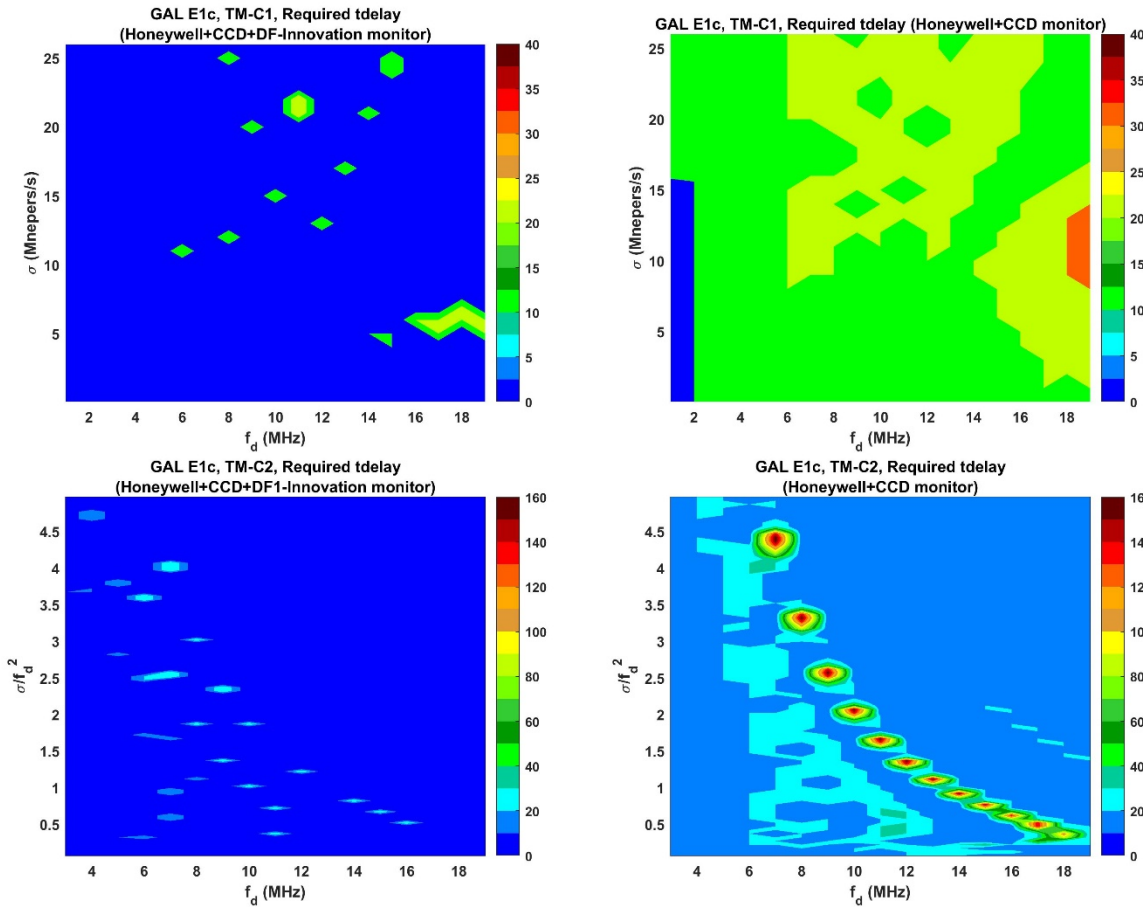
Fig. 15-Required tdelay for the PMD compliance for the TMC1 under Galileo E1c fault mode in the upper panel and TMC2 in the lower panel (left column: with the DF-Innovation monitor, right column: without the proposed monitor)
