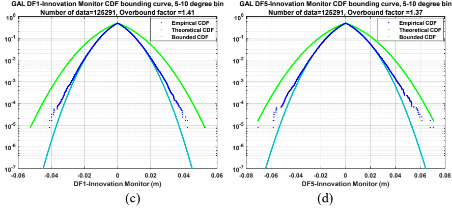
Fig. 5-The CDF of the DF-Innovation monitor for (a) GPS L1, (b) GPS L5, (c) Galileo E1 and (d) Galileo E5
