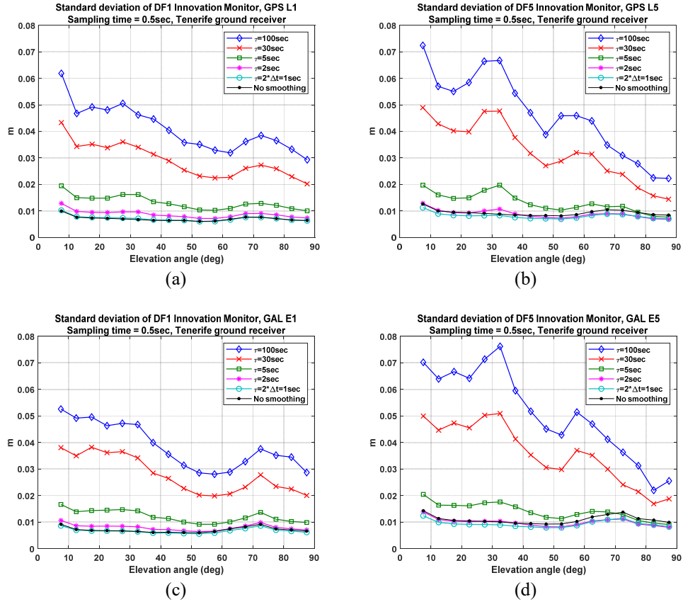
Fig. 4-The standard deviation of the DF-Innovation monitor for (a) GPS L1, (b) GPS L5, (c) Galileo E1 and (d) Galileo E5 signals at Tenerife ground receiver
