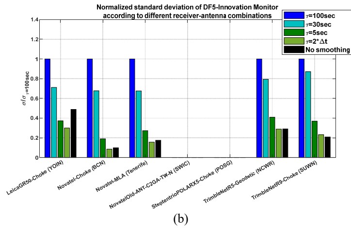
Fig. 2-Effect of different time constants of smoothing filter on the standard deviation of the DF-Innovation Monitor computed for elevation angles from 5 to 10 degrees for (a) L1 frequency and (b) L5 frequency (SWIC and POSG were not L5-frequency capable).
