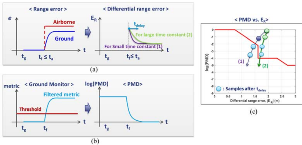
Fig. 10-Description of transient case and the effect of time constant of carrier smoothing for the PMD compliance:
