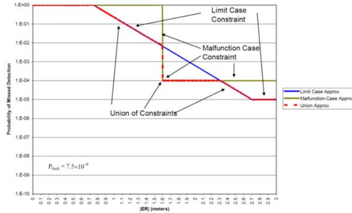
Fig. 6-The monitor PMD requirement for the CAT II/III in standards [3]
