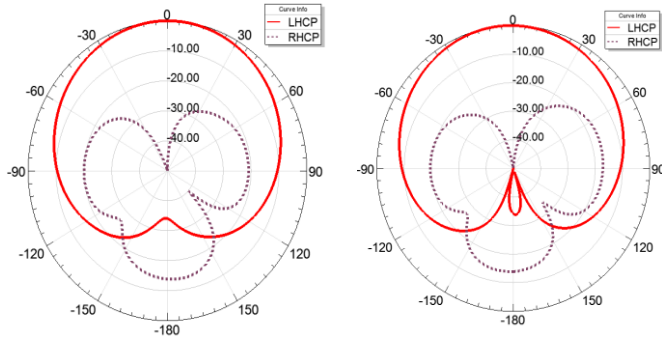
Fig. 7 Simulated normalized directivity of the ARDRA for LHCP and RHCP at f_o=2.45 GHz and \phi=0^\circ .
