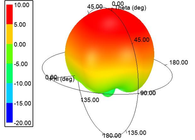
Fig. 8 Simulated 3D total directivity of the proposed ARDRA at f_o=2.45 GHz.
