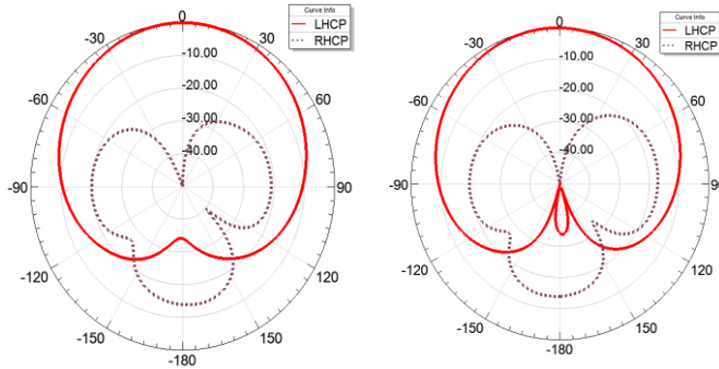
Fig. 7 Simulated normalized directivity of the ARDRA for LHCP and RHCP at f_o=2.45 , \theta=0^\circ and \phi=0^\circ .
