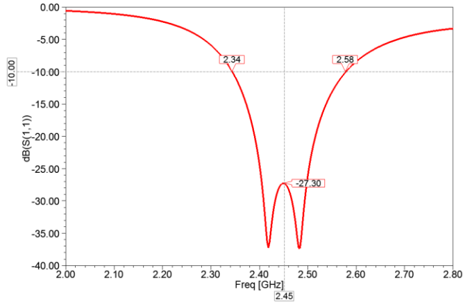
Fig. 3 Simulated S_{11} of the proposed ARDRA.
