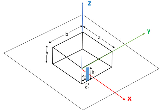
Fig. 1 Configuration of the ARDRA.
