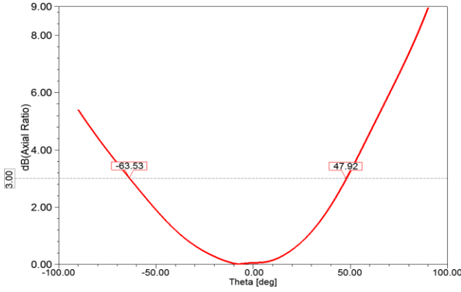
Fig. 6 Simulated axial ratio vs theta of the proposed ARDRA at f_o=2.45 GHz and \phi=0^\circ .
