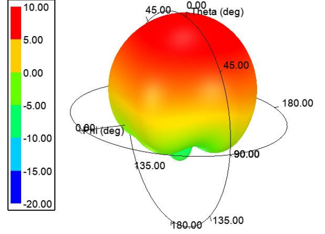
Fig. 8 Simulated 3D total directivity of the proposed ARDRA at f_o=2.45 .
