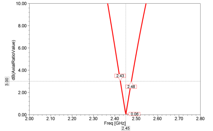
Fig. 5 Simulated axial ratio vs frequency of the proposed ARDRA at \theta=0^\circ and \phi=0^\circ .
