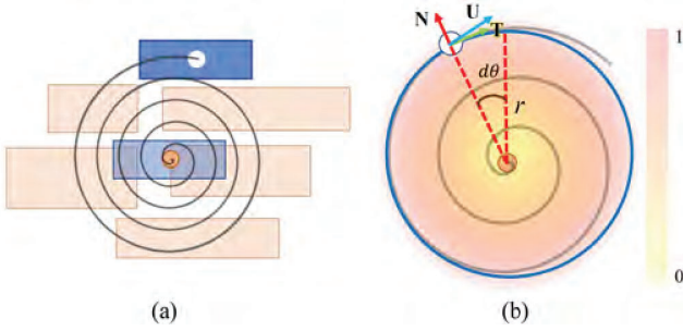
Fig. 3. (a) Along the spiral started from the orange dot, search for a position to place the next word (blue rectangle at the white dot), such that the word does not overlap with the existing words. (b) Illustrating the spiral movement direction U and the normal ( N ) and tangent ( T ) directions at the white point on the circle (in blue) of radius r . The circle can be taken as the isoline of the underlying scalar field from the origin, where the color map on the right reveals the scalar field magnitude ( r ).
