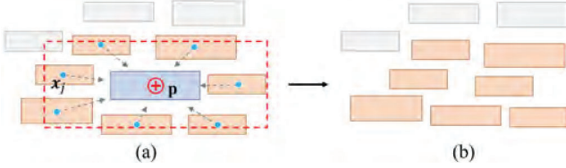
Fig. 10. Illustration of the uniform constraint: (a) central forces (grey arrows) towards the virtual rigid body in the middle, where the forces are applied to surrounding word boxes in the region marked by the red dashed box; and (b) updated layout, where the position of surrounding word boxes are re-adjusted.
