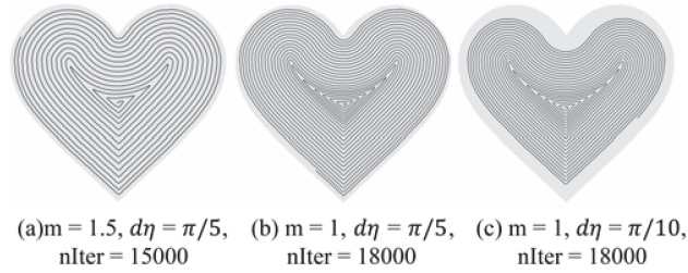
Fig. 5. Examples of shape-aware Archimedean spirals generated on the same shape using different parameters m , d\eta , and number of iterations (nIter).
