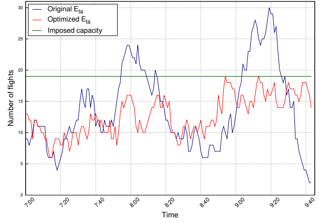
Figure 8. Comparison of taxiway network occupancy
