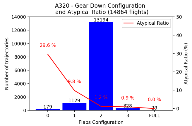
Figure 13: This figures displays the landing gear action appearance distribution in the landing sequence and the atypical ratio correlation for all the A320 flights
