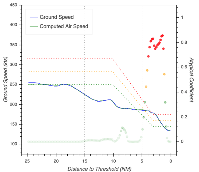
Figure 8: The third graph of TAPAS section Flight Study, displaying the ground speed and computed air speed profile. The colored dots corresponds to the atypical coefficients between nominal (0 and green) and atypical (1 and red).
