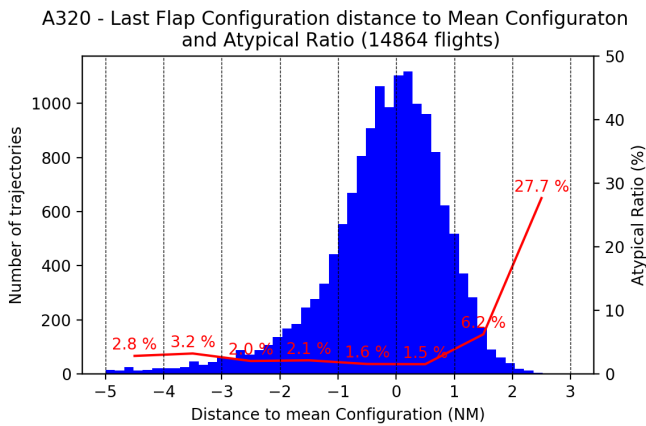
Figure 14: This figures shows last landing configuration element distance to the mean distribution and the atypical ratio correlation for all the A320 flights
