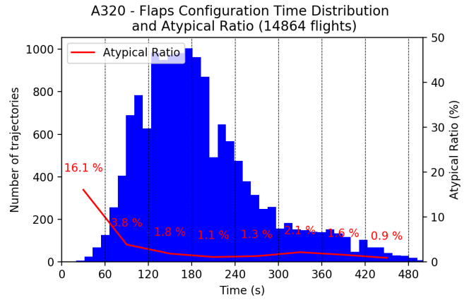
Figure 12: This figures illustrates landing configuration time distribution and atypical ratio correlation for all the A320 flights
