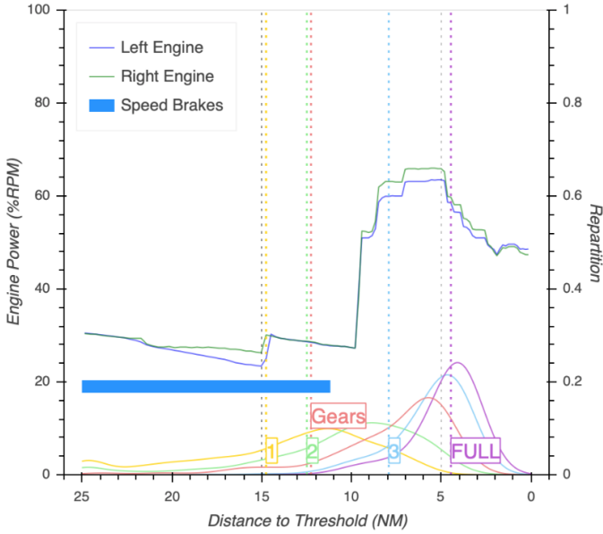
Figure 9: The fourth graph of TAPAS section Flight Study, displaying the engine power, the flaps settings, the landing gear setting, and the airbrake use. (The Gaussian curves illustrate the distribution of configuration elements for all the flights with this specific runway QFU)
