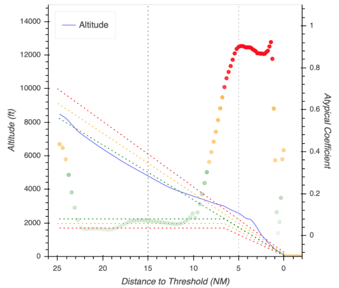
Figure 7: The second graph of TAPAS section Flight Study, displaying the altitude profile. The colored dots corresponds to the atypicality coefficients between nominal (0 and green) and atypical (1 and red).
