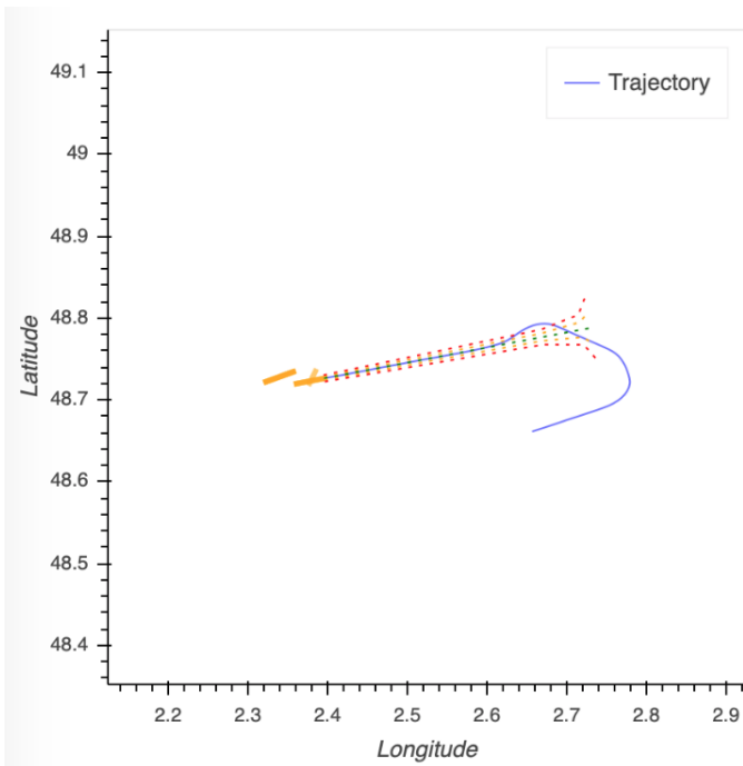
Figure 6: The first graph of TAPAS section Flight Study, displaying the longitudinal path and lateral compliance criteria
