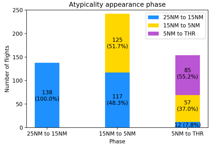
Figure 10: An illustration of the atypicality appearance phase
