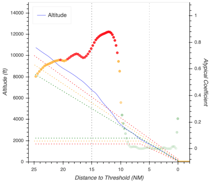
Figure 11: An example of an atypical flight during phase 25NM to 15NM and 15NM to 5NM
