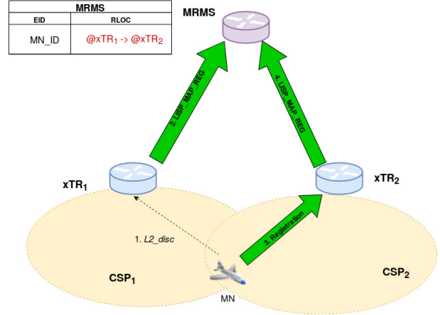
Fig. 3. LISP Handoff Management
