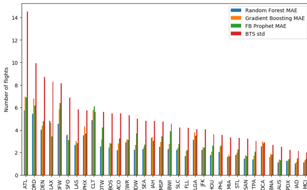
Figure 2: Comparison of the mean absolute errors per airport for the trained regressors for the estimation of the number of delayed departing flights. The standard deviation of the BTS value on the training set is included for comparison.
