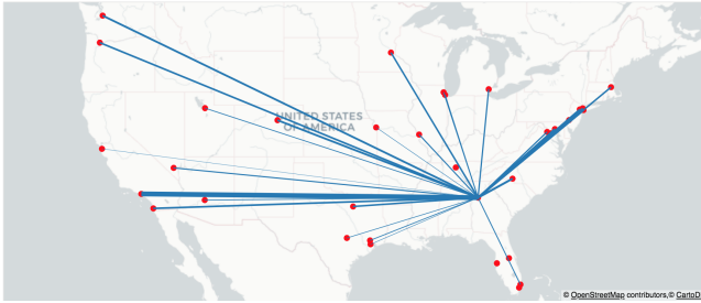
Figure 7: Map of feature links between Atlanta airport (ATL) and the other airports for estimating the number of delayed departing flights. The larger the link, the more features were kept among the features gathering 99% of the total importance for estimating the number of departing delayed flights at ATL.
