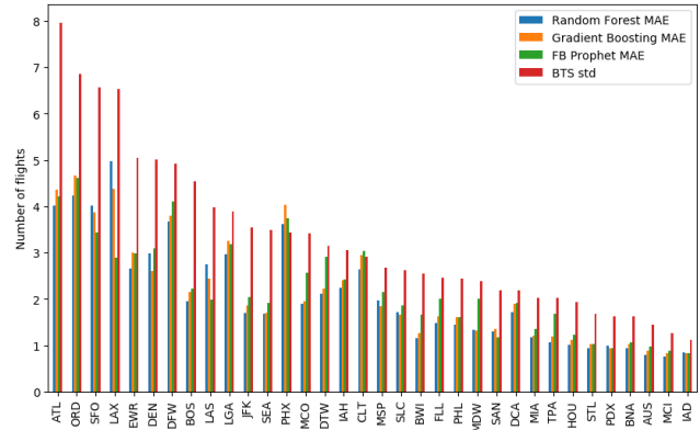
Figure 3: Comparison of the mean absolute errors per airport for the trained regressors for the estimation of the number of flights arriving with a delay greater than 15 minutes. The standard deviation of the BTS value on the training set is included for comparison.
