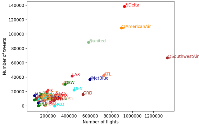
Figure 1: Number of tweets over the number of flights during the year 2017 for the considered airlines and airports
