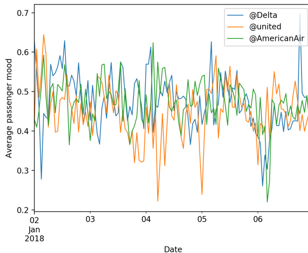
Figure 6: Average passenger sentiment with respect to three major airlines over the period January 2nd, 2018 to January 6th, 2018, corresponding to a bomb cyclone hitting in the North-East of the US.
