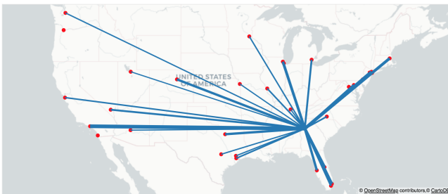
Figure 8: Map of delay links between Atlanta airport (ATL) and the other airports. The larger the link, the more flights departed with a delay during 2017 from ATL towards the connecting airport. Only links with more than 1000 delayed flights in 2017 were considered.
