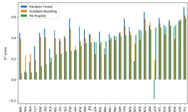
Figure 4: Comparison of the R^2 scores per airport for the trained regressors for the estimation of the number of delayed departing flights
