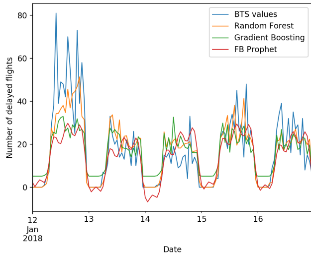
Figure 5: Predicted number of delayed departing flights at ATL by the trained regressor over the period January 12th, 2018 to January 16th, 2018. The actual number of delayed departing flights is indicated for comparison.
