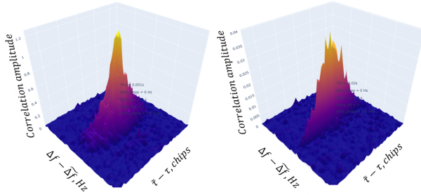
Figure 4: Synthetic correlator output visualization for T_{int} = 1 ms (left) and T_{int} = 20 ms (left)
