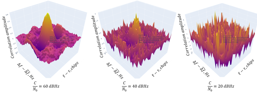
Figure 5: Synthetic correlator output visualization for I-channel for different values of carrier-to-noise ratio
