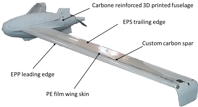
Figure 6: UAV construction.
