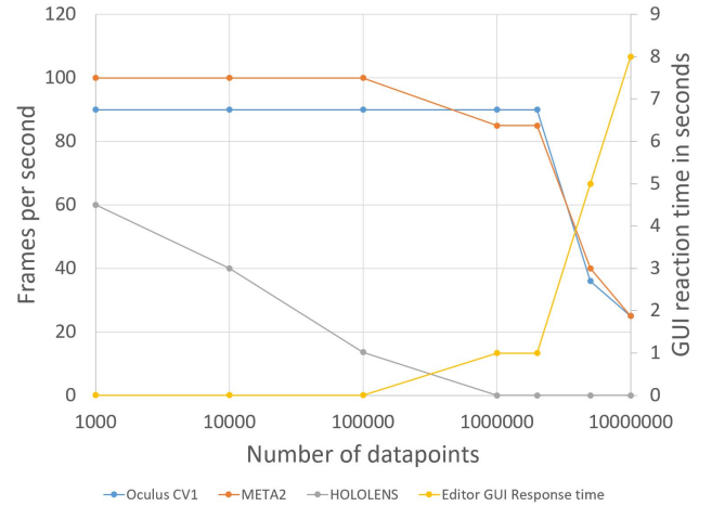
Figure 5: IATK FPS and editor response time performances
