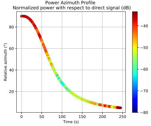
Fig. 6: Power Azimuth Profile of the multipath along the trajectory.
