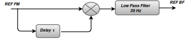
Fig. 3: Block diagram of the FM demodulator.
