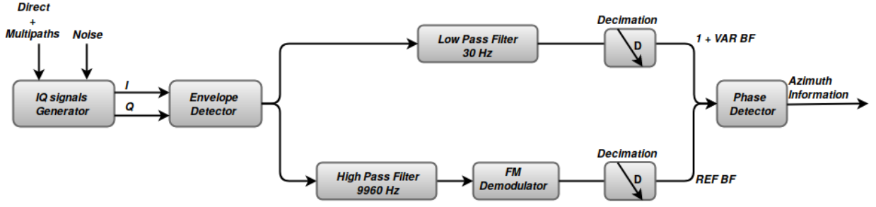
Fig. 2: Block diagram of the VOR receiver.
