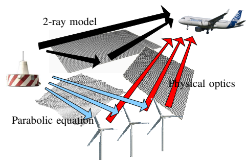
Fig. 1: Overview of the method to compute multipath [3].
