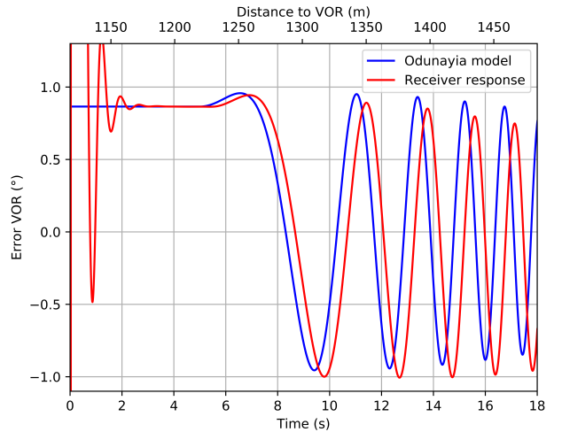
(b) Receiver response from 0 s to 18 s
