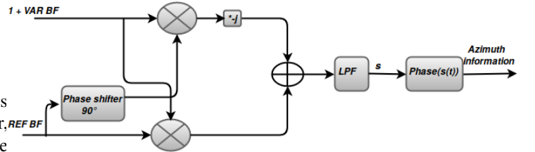
Fig. 4: Block diagram of the phase detector.
