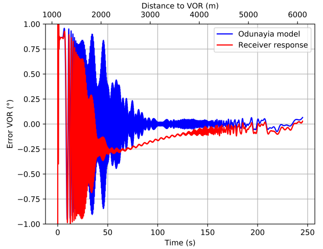
(a) Receiver response from 0 s to 250 s
