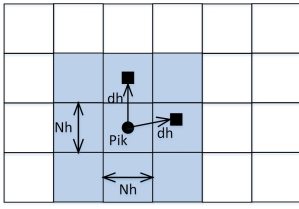
(a) Detect the conflicts in the horizontal plane by checking all neighborhood cells.
