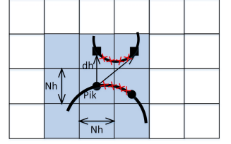
(d) Check the conflicts between two neighbored trajectory samples using time interpolations. Several trajectory samples (red crosses) are generated.
