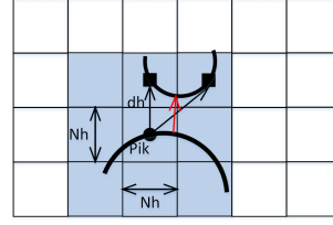
(c) Some conflicts between two neighbored trajectory samples may not be detected (the red arrow). It is necessary to check them.
