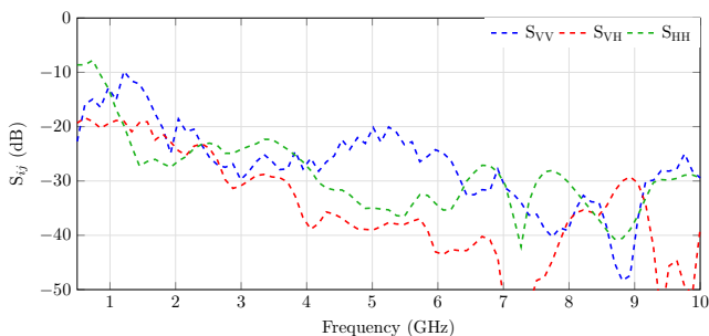
Fig. 3. Measured isolation between the vertical (V) or/and horizontal (H) ports of the Four Season VA as a function of frequency. Only the highest (i.e., worst-case) mutual couplings S_{ij} are plotted.
