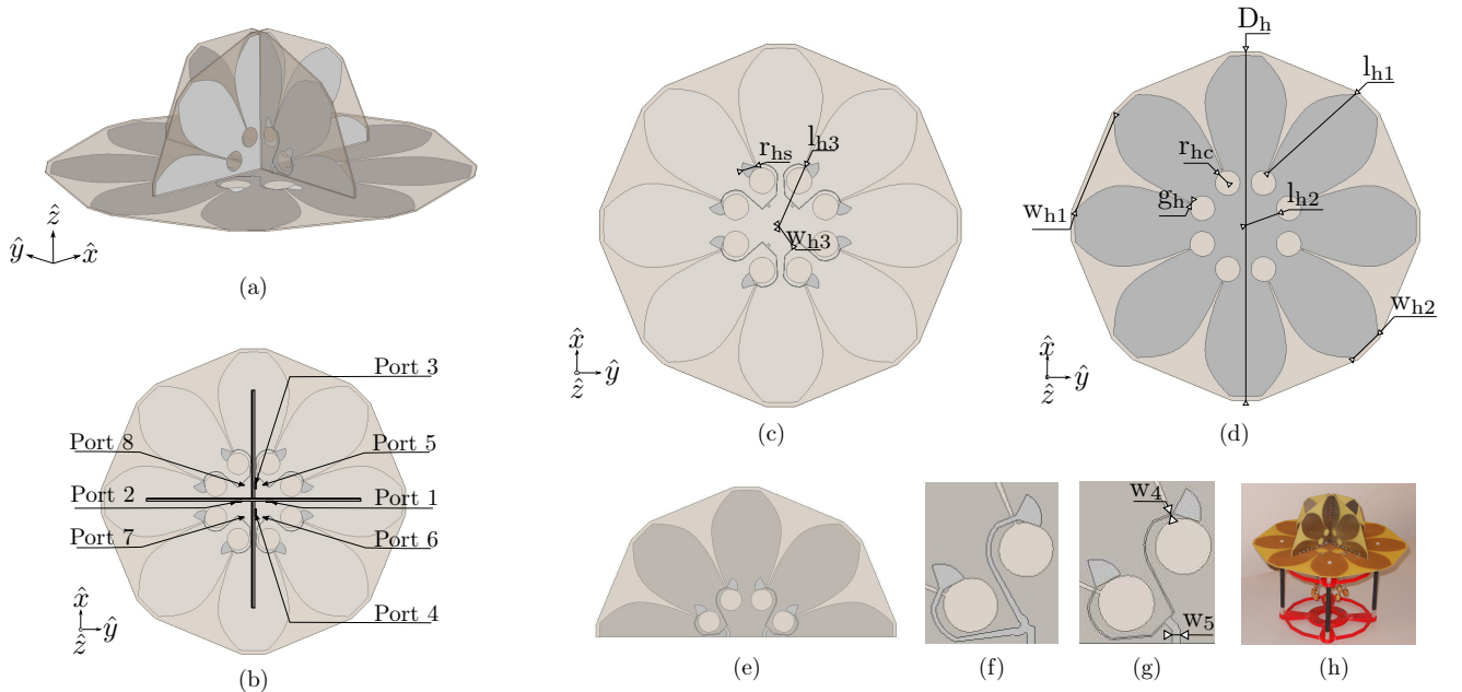
Fig. 1. Geometry (a), ports numbering (b), and fabricated prototype (h) of the Four Season VA. Top (c) and back (d) views of the horizontal part constituting the VA. Geometry of the vertical arrays of the VA (e) with a zoom on the previous (f) and new (g) feeding circuits.
