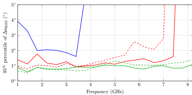
Fig. 5. Simulated (solid line) and measured (dashed line) 95 th percentile of \Delta a_{\text{RMS}} obtained from the Four Season VA for the estimation of the: (a) vertically- (red line) or (b) horizontally-polarized (green line) EM field using RPC 00. The blue line corresponds to the DoA estimation accuracy of the vertically-polarized EM field achieved from RPC 0.
