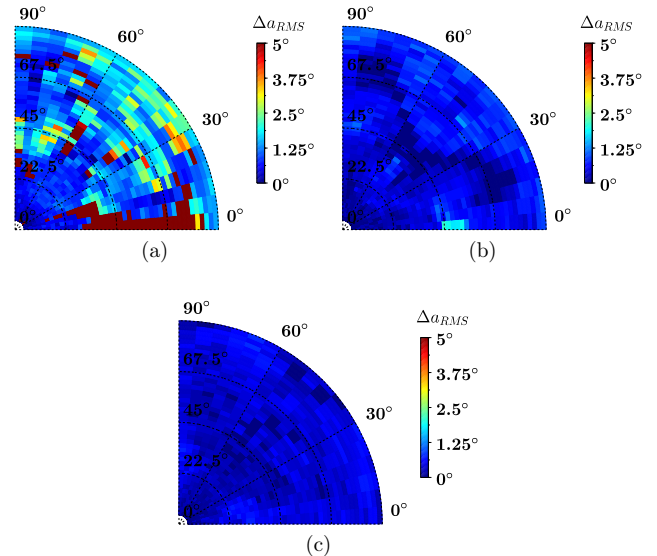
Fig. 6. Measured \Delta a_{\text{RMS}} at 3.8 GHz obtained from the Four Season VA using (a) RPC 0 or (b&c) RPC 00 for the estimation of the: (a&b) vertically- or (c) horizontally-polarized EM field.
