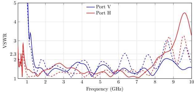
Fig. 2. Simulated (solid line) and measured (dashed line) VSWR of the Four Season VA as a function of frequency. For symmetry reasons, only measurement at one vertical (V) port and one horizontal (H) port are plotted.
