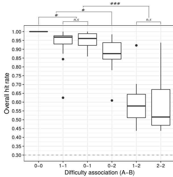
Figure 2. Overall hit rate per difficulty association. Boxplot with whisker bold band represents median values of hit rate. The upper and lower end of the boxes represent 95% confidence intervals. Whiskers represent ranges. Points are outliers. ( n.s. : not significant, * < .05 , *** < .001 )
