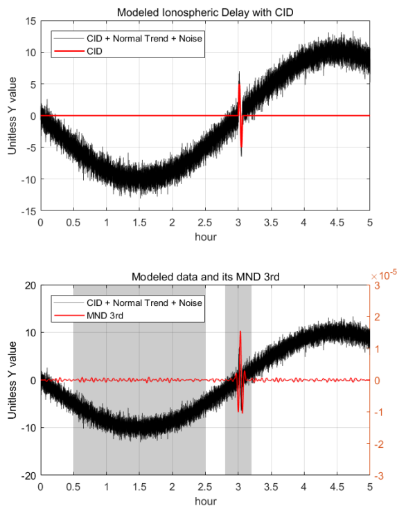
Fig. 2. Modeled ionospheric delay with CID (black), pure CID (top, red) and MND 3 rd of modelled data (bottom, red). Shades represent the regions from which STD and maximum absolute value were calculated respectively.
