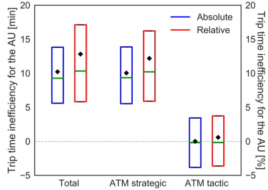
Figure 5. Trip-time-based flight inefficiency (Jul 28 th 2016, FABEC)
