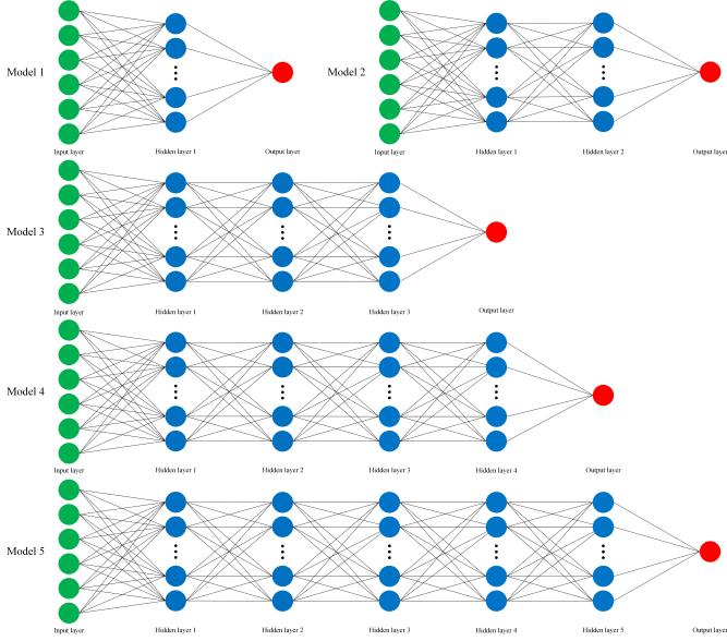
Figure 7: Structures of 5 NNs model used in this paper
