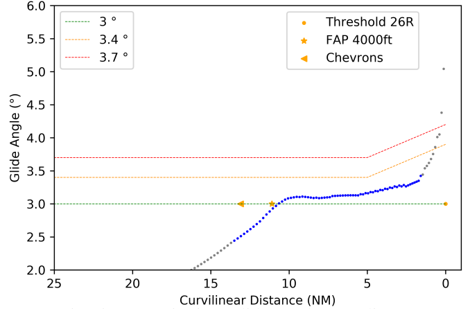
Fig. 5: New criteria : Glide Angle compliance
