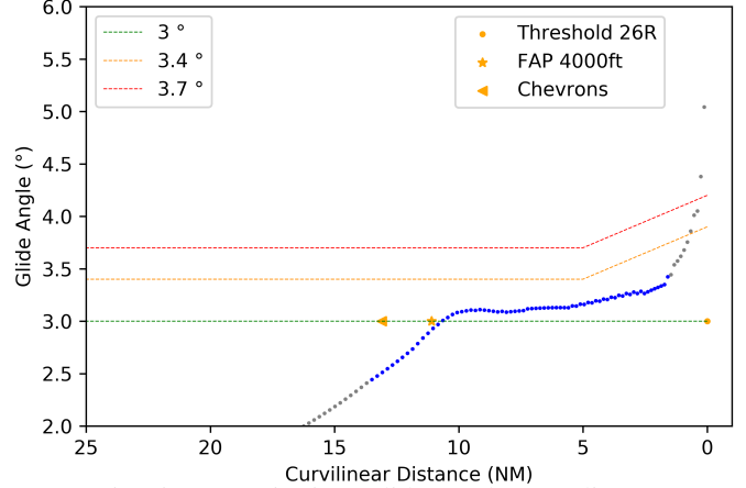
Fig. 5: New criteria : Glide Angle compliance
