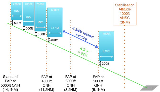
Fig. 2: Illustration of the Area Proximity Warning set up at CDG
