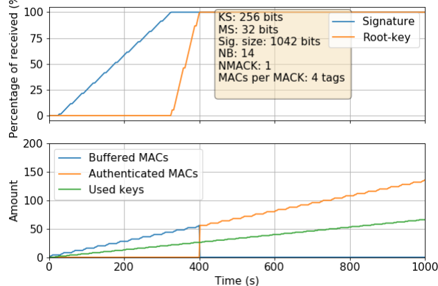
Figure 7 – Time-sequence of signature, root-key, and MAC reception for the slowest possible TTFAF.
