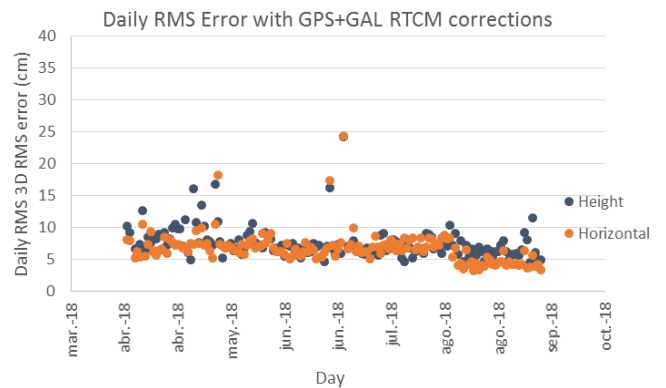
Figure 44 – Daily RMS with GPS+GAL (RTCM)
