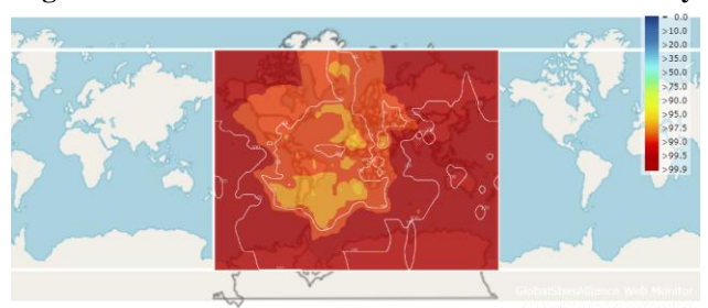
Figure 37 – 09/06/2018 SBAS L5 LPV-200 Availability
