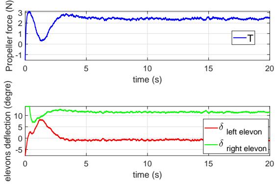
Figure 10: Control U
